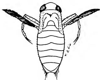
Fig. 357. Arctocorixa alternata Say, 5th instar.
